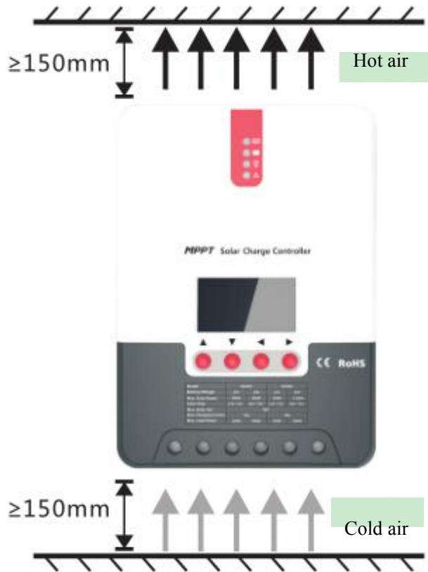
Fig. 2.1 Installation and heat dissipation
